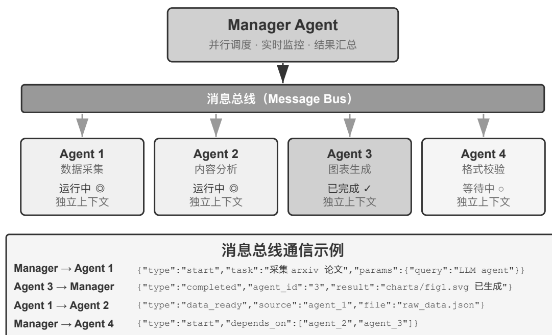
图 10-7 Manager 并行协调
